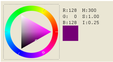
IupDial
