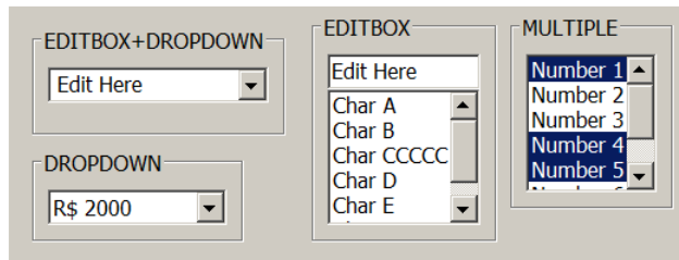
Windows XP
